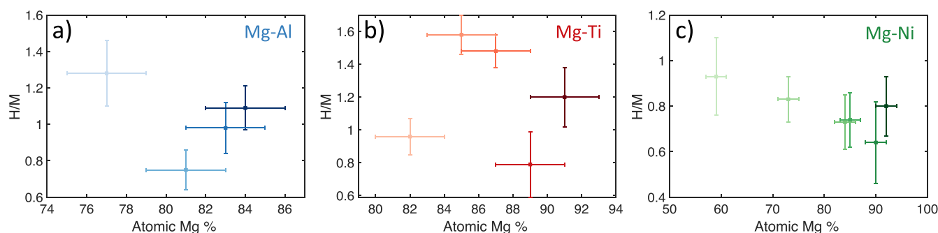
Figure 8. Measured maximum loading values under 1 bar \text{H}_2 for different thin films for (a) \text{Mg-Al} , (b) \text{Mg-Ti} , and (c) \text{Mg-Ni} alloy samples. The horizontal and vertical error bars represent one standard deviation uncertainty in the atomic \text{Mg} % and the loading, respectively.
